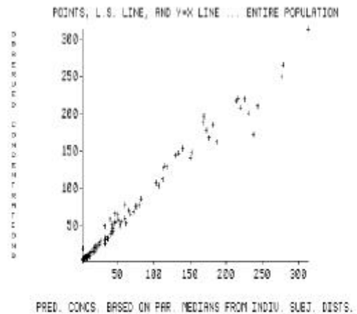
Fig 15. Scattergram of estimated serum concentrations based of individual subject Bayesian posterior median values.
