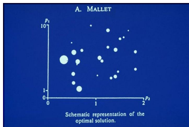
Figure 1. An example of an NP population model made by Mallet. Horizontal axis, a parameter such as the rate constant for elimination. Vertical axis, a parameter such as apparent volume of distribution. Note the clearly non-Gaussian shape of the horizontal parameter, with the central gap. This may well represent two unsuspected subpopulations such as fast and slow metabolizers of a drug. The size of each point reflects its estimated probability (reproduced by permission).
