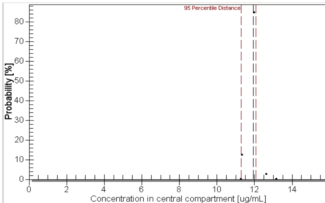
Figure 6. Profile of the multiple predictions at the time of the first peak achieved on the new regimen. Horizontal = the multiple predicted serum concentrations. Vertical = probability of each prediction. Middle dashed vertical line = predicted weighted average concentration of 11.93 ug/mL (target = 12). Outer dashed lines = 95 percentile distributions (roughly 11.3 to 12.2 ug/mL) of the predictions. Note the much narrower bandwidth of the 95% distance of predictions around the predicted peak serum concentration of 11.93 ug/mL, Compare this figure with Figure 4 above.
