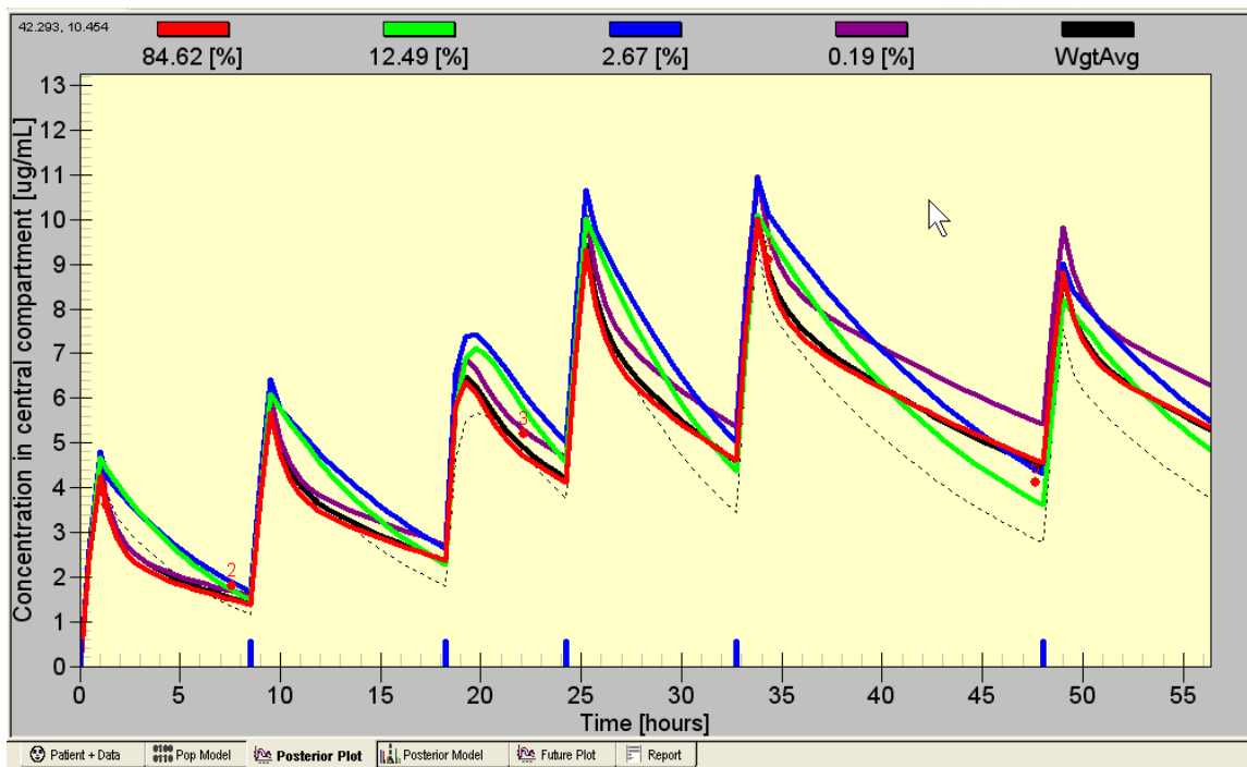
Figure 5. Plot of the trajectories of estimated serum concentrations produced by MM Bayesian analysis of the above patient's data. Instead of 76 estimations as shown in the population PK model in Figure 4, only 5 support points survived the Bayesian analysis. Note their very much increased probabilities, up to 84%, (top horizontal of the figure) compared to those of the population model, where the highest probability of the various support points was 13%. The five measured serum concentrations are shown by the round dots and their nearby numbers.
