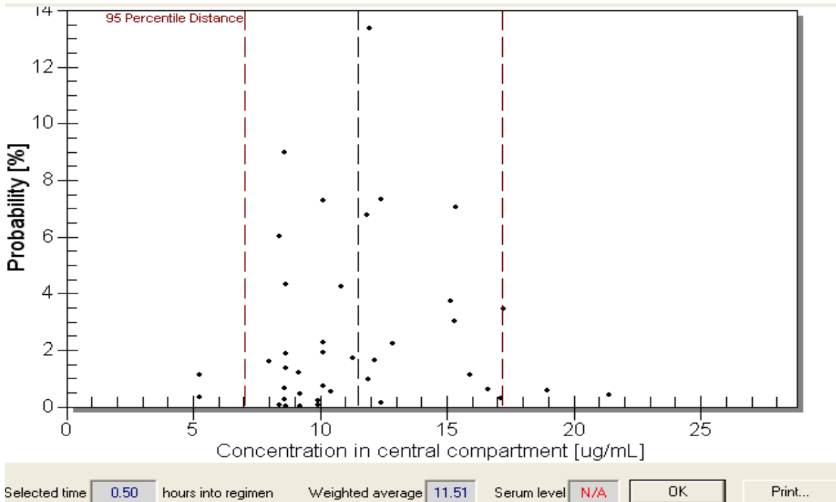
Figure 4. Time slice of the multiple predictions at \frac{1}{2} h into the regimen, the time of the peak serum concentration. Horizontal = the multiple predicted serum concentrations. Vertical = probability of each prediction. Middle dashed vertical line = predicted weighted average concentration of 11.51 ug/mL (target = 12). Outer dashed lines = 95 percentile distributions (roughly 7 to 17 ug/mL) of the predictions.
